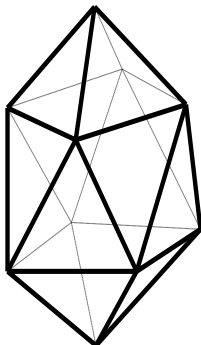
Hexacaidecahedron
